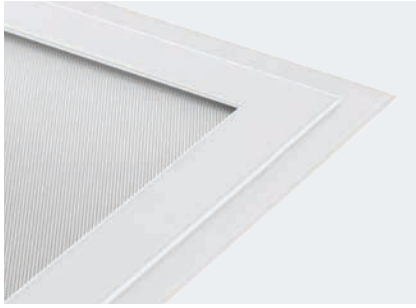
Microprismatic cover. The structured surface is homogeneous at a viewing distance of 50 cm or more.
